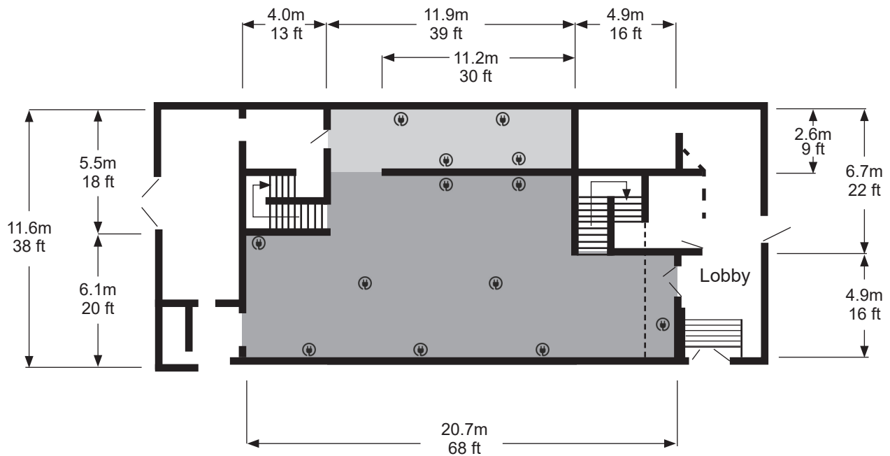
Ground Floor Exhibition Area
