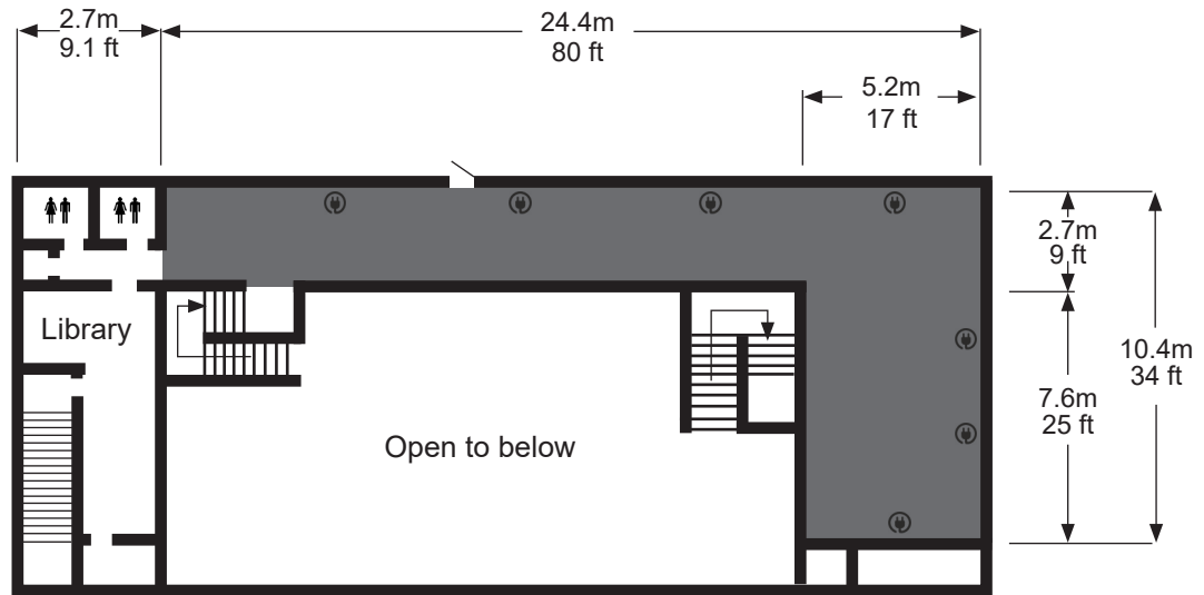
Mezzanine Exhibition Area
